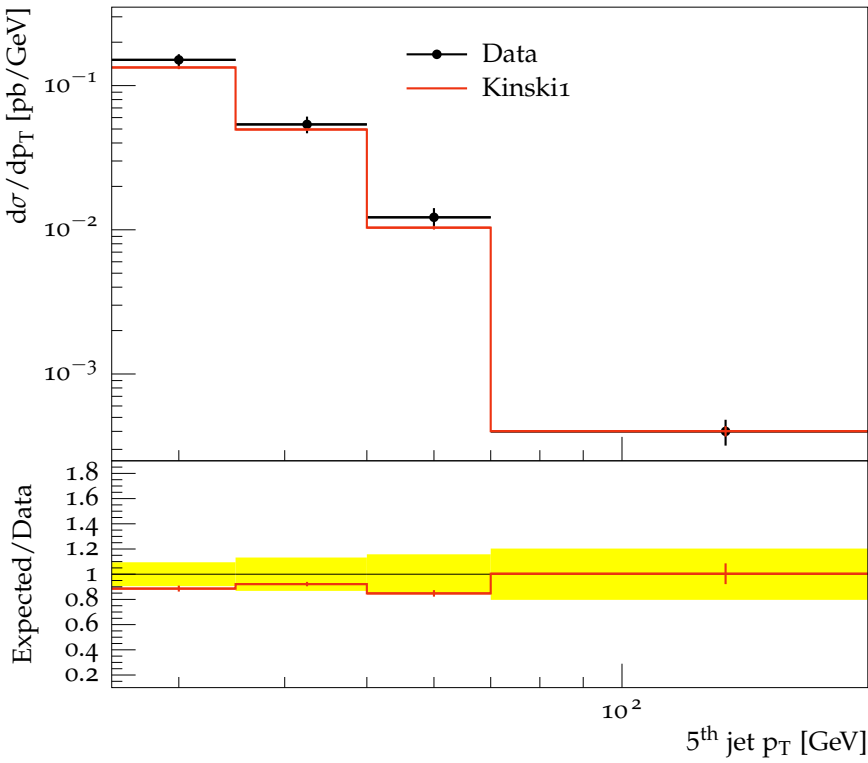
t\bar{t} cross-section vs. 5 th jet p_T
