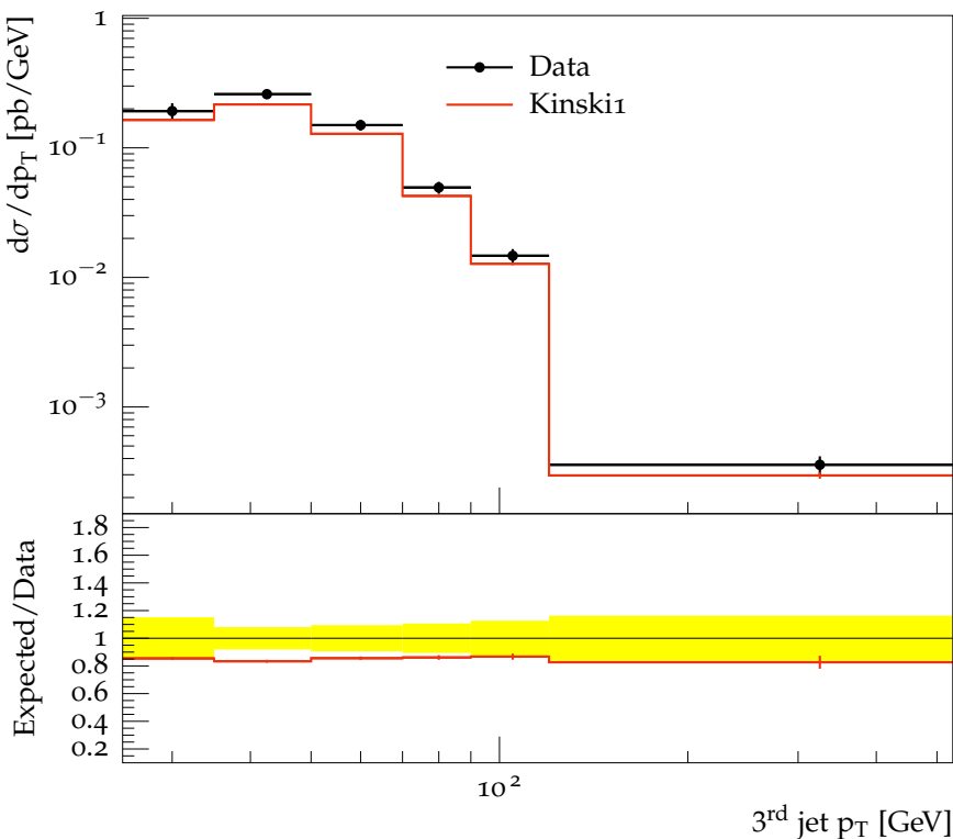
t\bar{t} cross-section vs. 3 rd jet p_T
