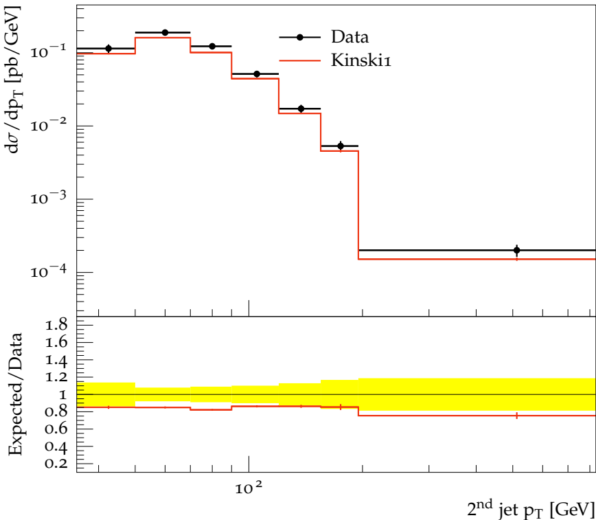
t\bar{t} cross-section vs. 2 nd jet p_T
