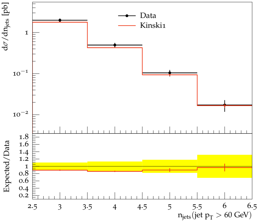
t\bar{t} cross-section vs. jet multiplicity for jets above 60 GeV
