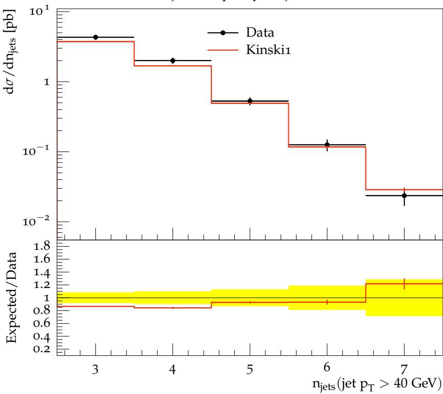
t\bar{t} cross-section vs. jet multiplicity for jets above 40 GeV
