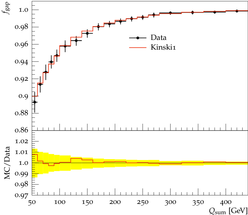
Gap fraction vs. Q_{\text{sum}} for veto region: 0.8 < |y| < 1.5
