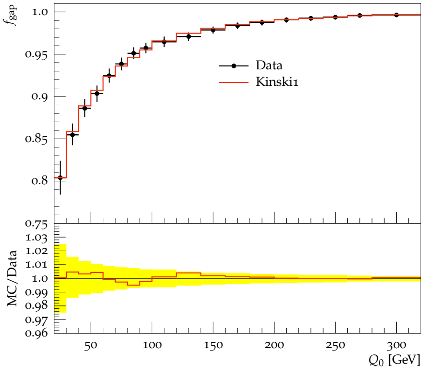
Gap fraction vs. Q_0 for veto region: 0.8 < |y| < 1.5
