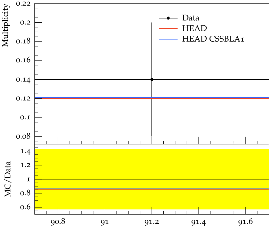
Mean f_0(980) multiplicity
