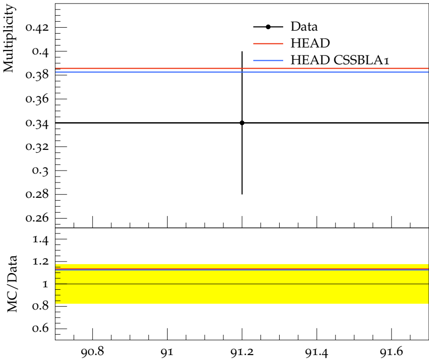
Mean B^+ / B^- / B^0 multiplicity
