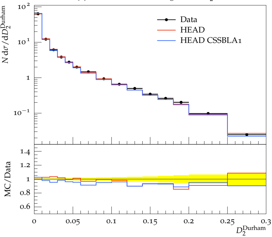
Differential 3-jet rate with Durham algorithm, D_2^{\text{Durham}}
