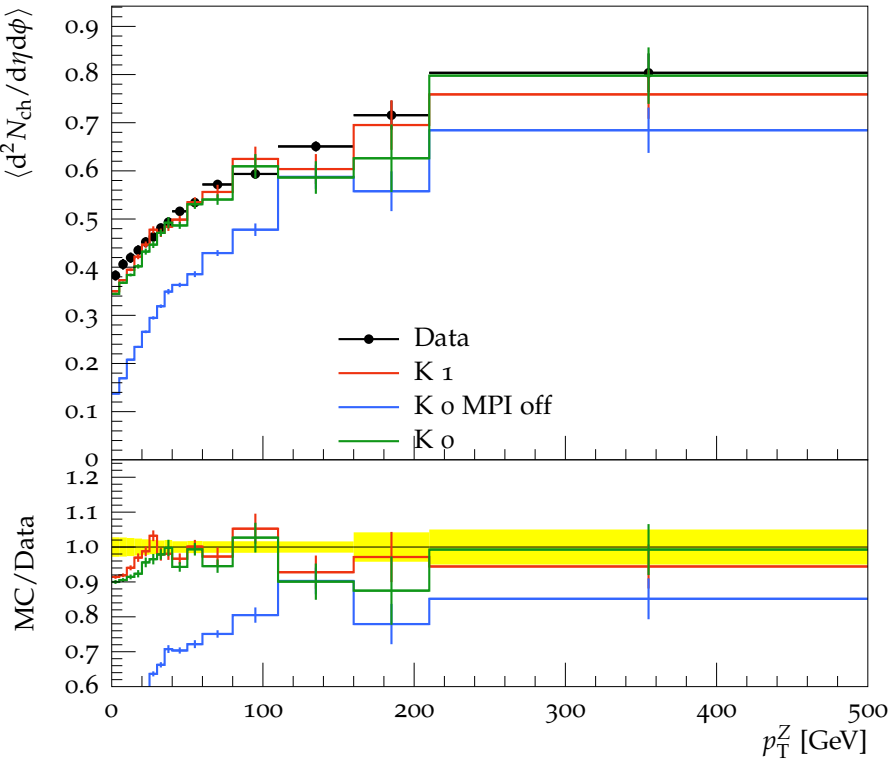
Trans-diff region, dressed level
