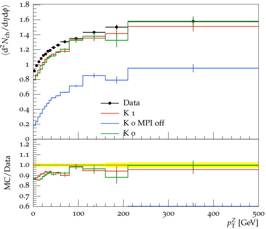
Trans-max region, dressed level
