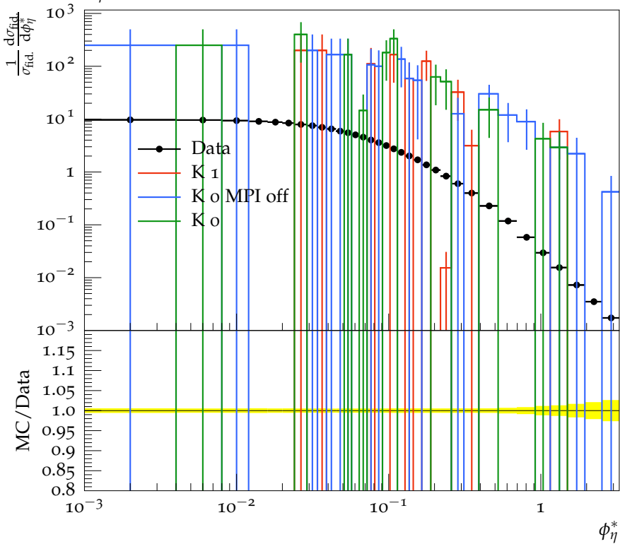
\phi_\eta^* spectrum, Z \rightarrow e\bar{e} (dressed)
