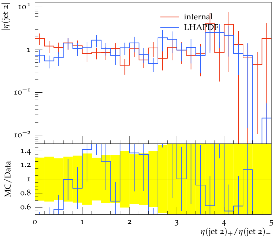
Pseudorapidity \pm ratio of second jet
