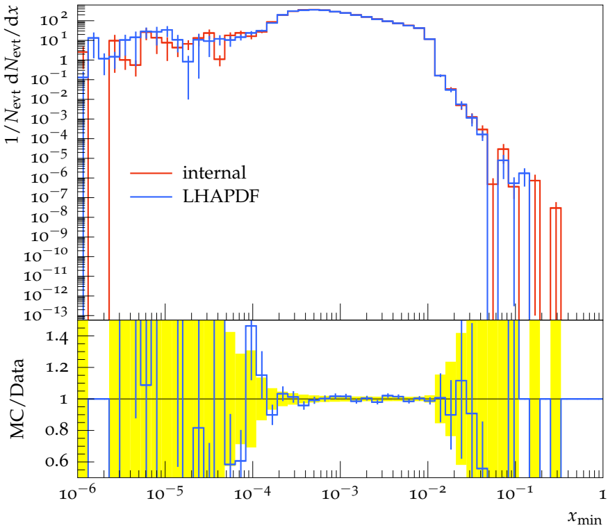
PDF sampling x_{\min} value distribution
