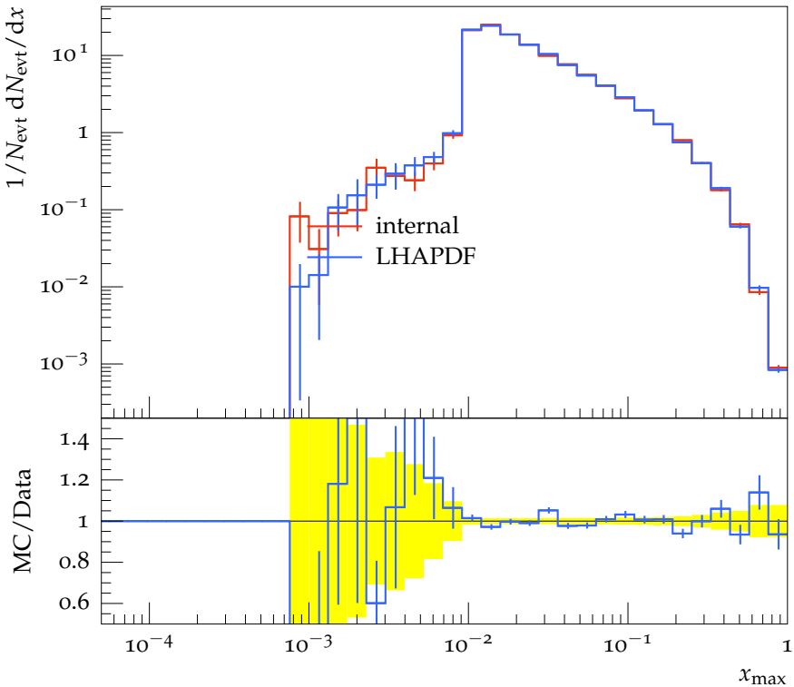
PDF sampling x_{\max} value distribution
