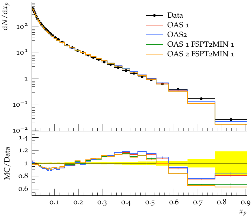
Charged particle scaled Momentum, ( uds ) events
