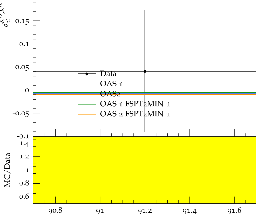
Multiplicity difference b\text{-}uds for K^{*0}, \bar{K}^{*0}
