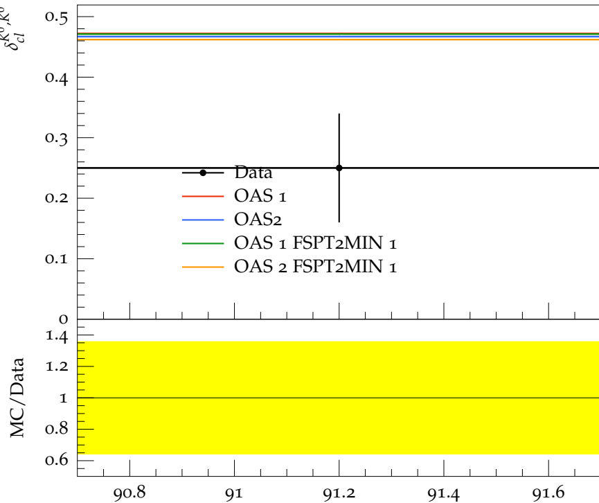
Multiplicity difference b \rightarrow uds for K^0, \bar{K}^0
