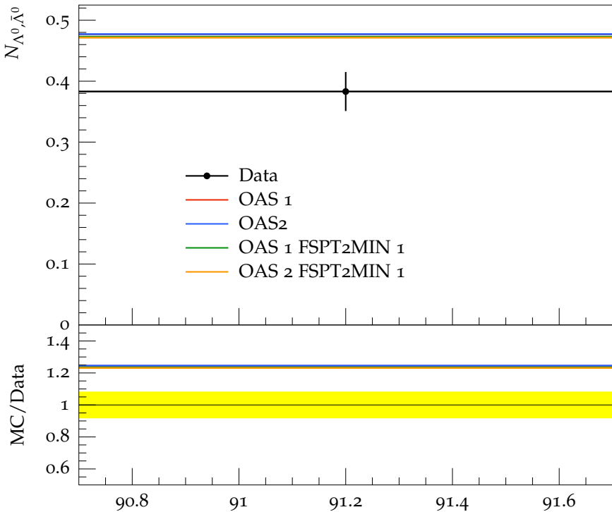
Multiplicity of \Lambda^0, \bar{\Lambda}^0 in b events
