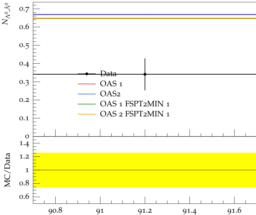
Multiplicity of \Lambda^0, \bar{\Lambda}^0 in c events
