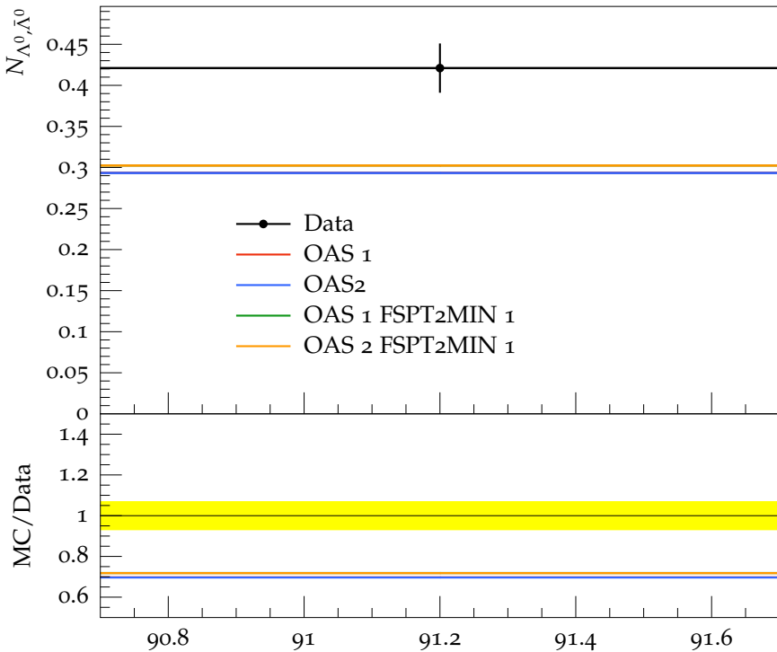
Multiplicity of \Lambda^0, \bar{\Lambda}^0 in ( uds ) events
