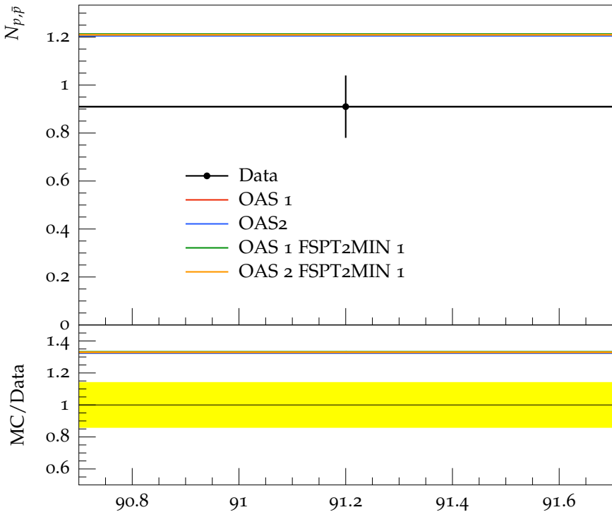
Multiplicity of p, \bar{p} in b events
