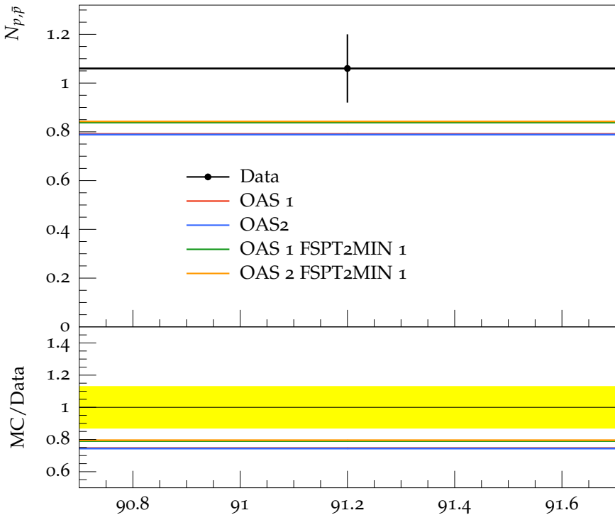
Multiplicity of p, \bar{p} in ( uds ) events
