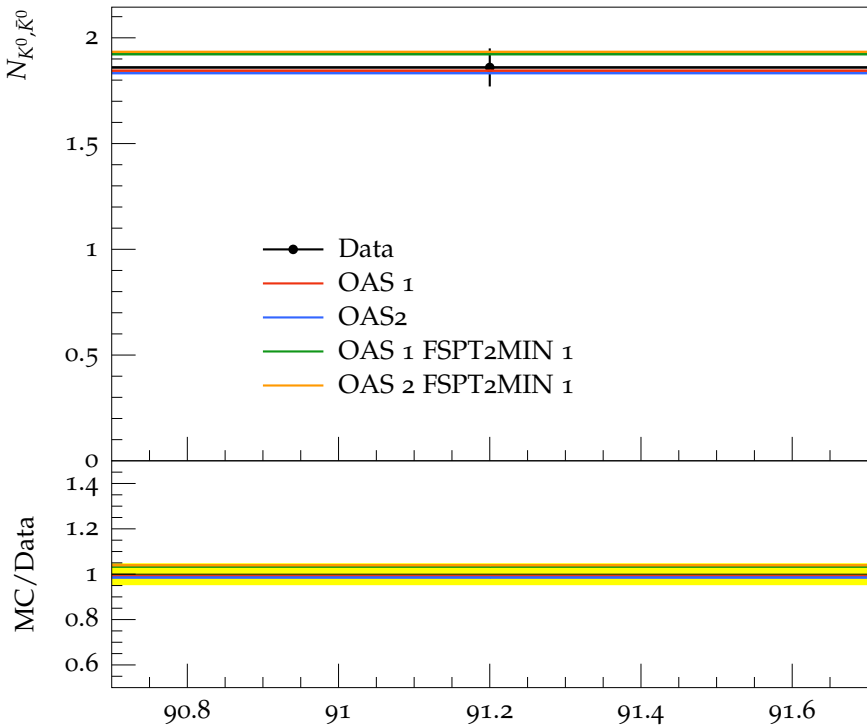
Multiplicity of K^0, \bar{K}^0 in ( uds ) events
