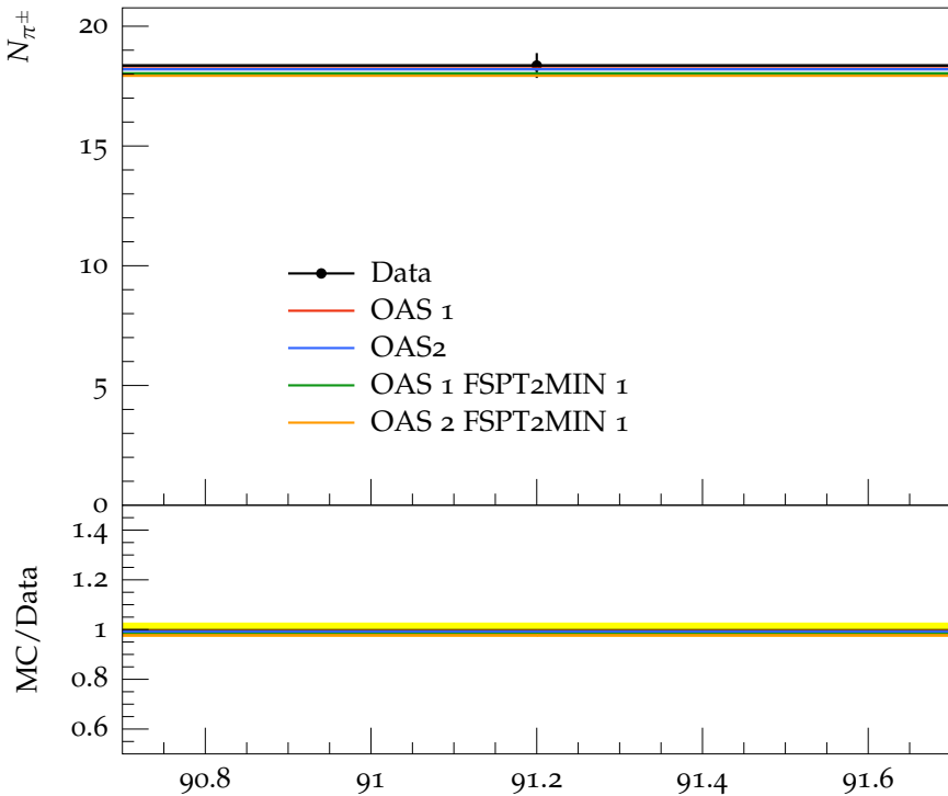
Multiplicity of \pi^\pm in b events
