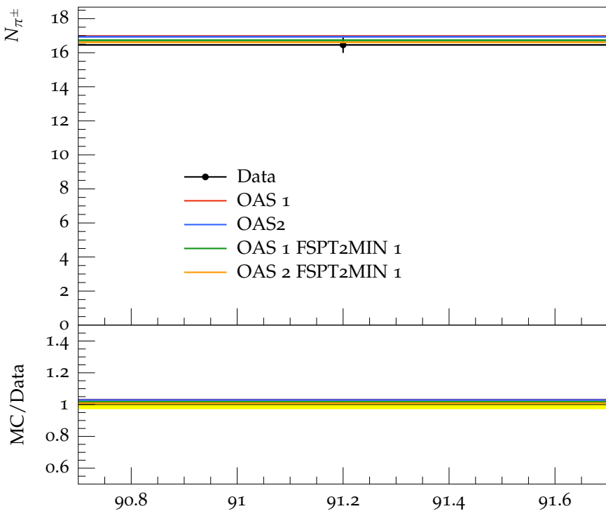
Multiplicity of \pi^\pm in ( uds ) events
