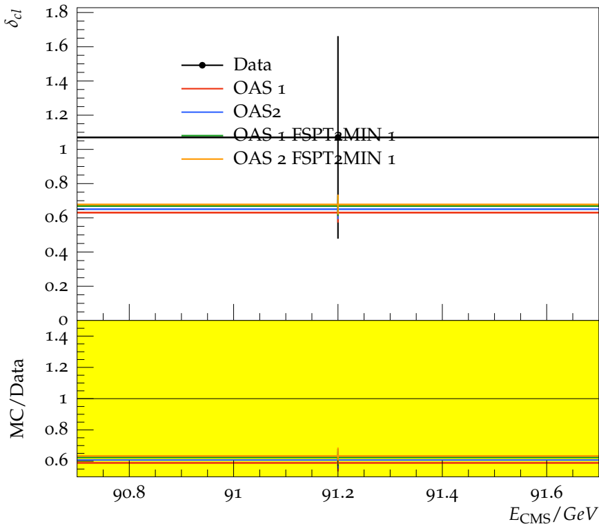
Difference in Charged multiplicity between c and uds events
