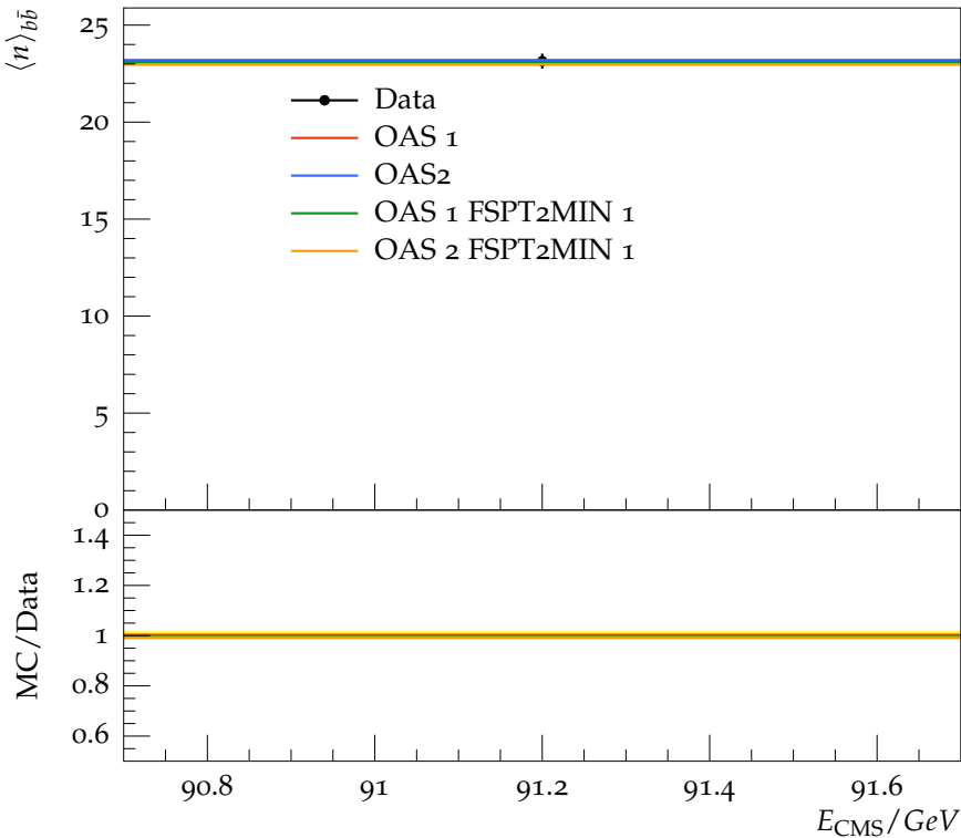
Charged multiplicity in b events
