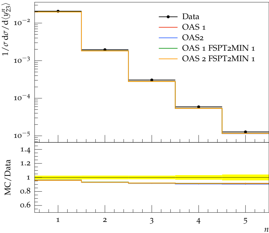
Moments of y_{23} at 91 GeV
