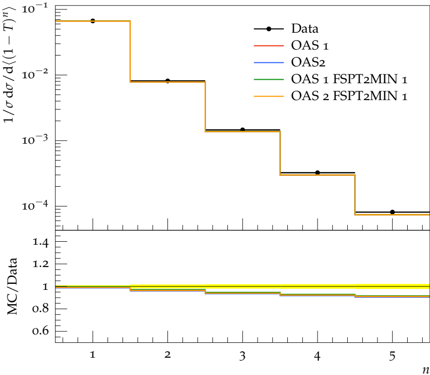
Moments of 1 - T at 91 GeV
