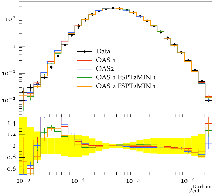
Integrated 5-jet rate with Durham algorithm (91.2 GeV)
