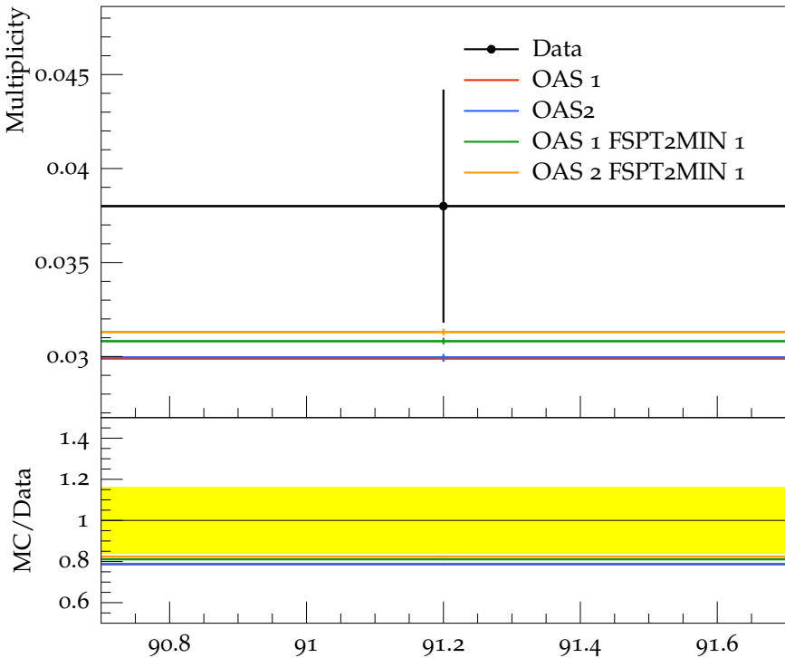
Mean \Sigma(1385)^+/\Sigma(1385)^- multiplicity
