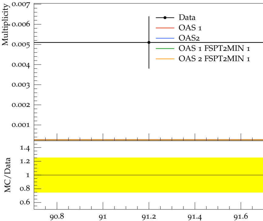
Mean \Omega^- multiplicity
