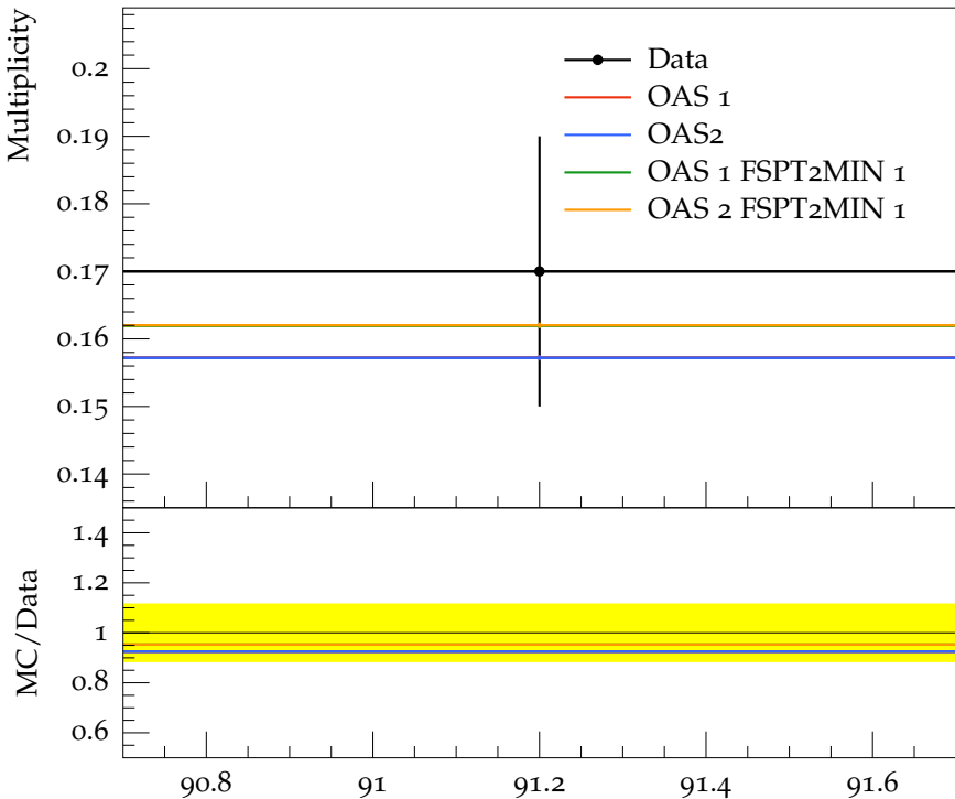
Mean D^*(2010)^+/D^*(2010)^- multiplicity
