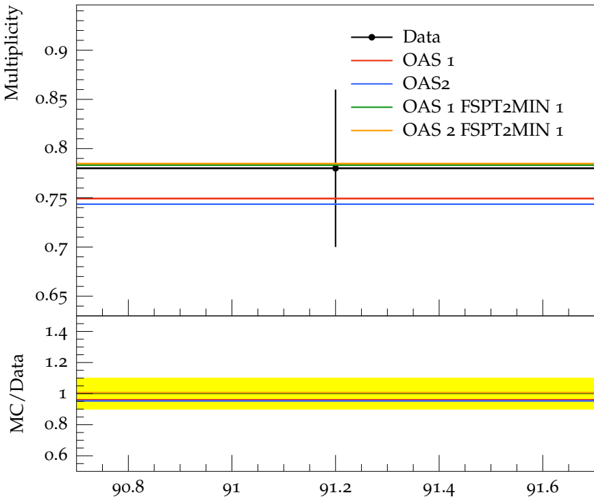
Mean K^*(892)^+ / K^*(892)^- multiplicity
