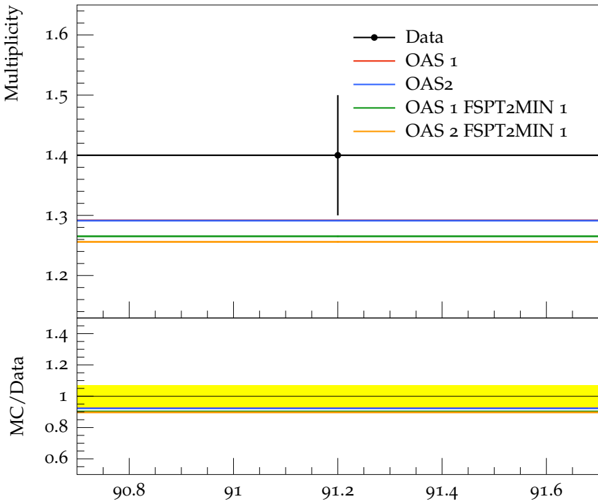
Mean \rho multiplicity
