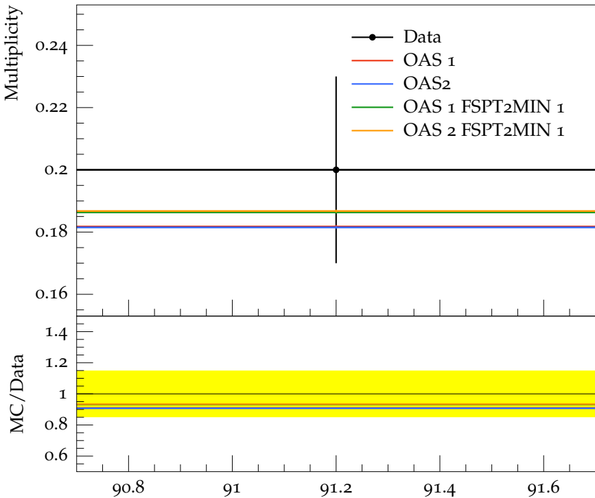
Mean D^+ multiplicity
