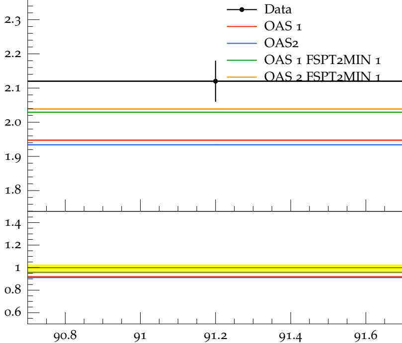
Mean K^0 multiplicity
