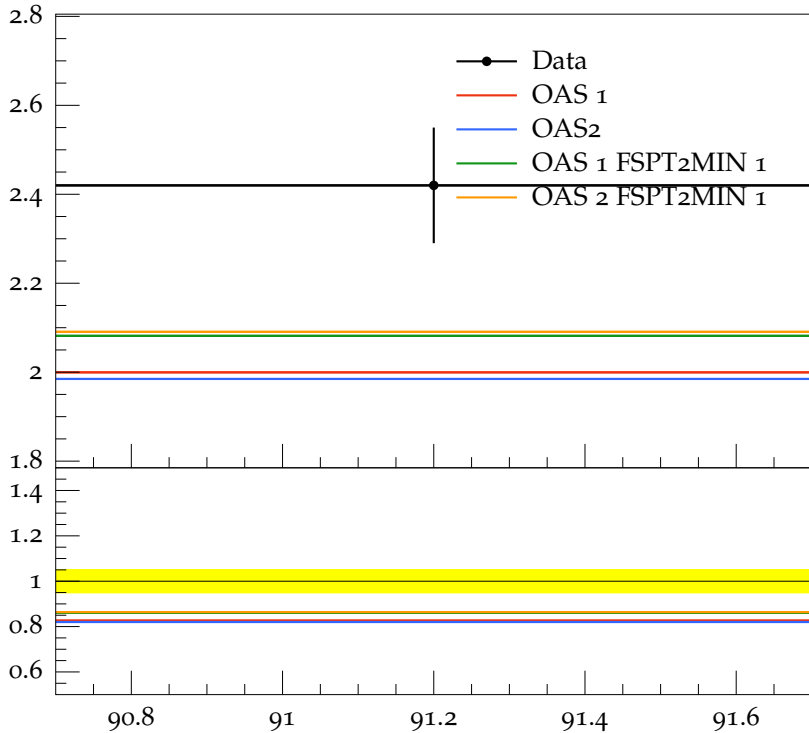
Mean K^+ / K^- multiplicity
