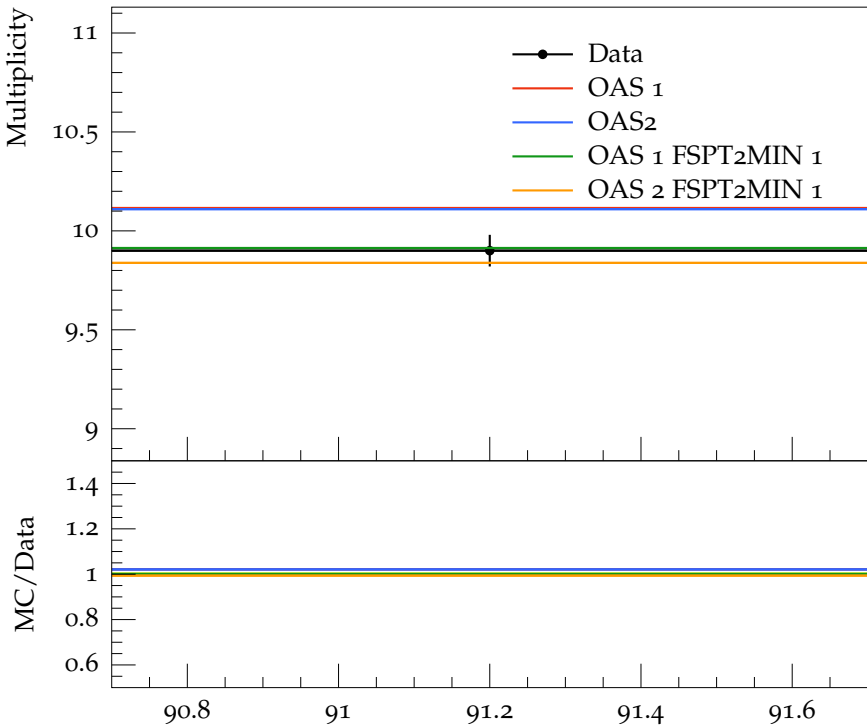
Mean \pi^0 multiplicity
