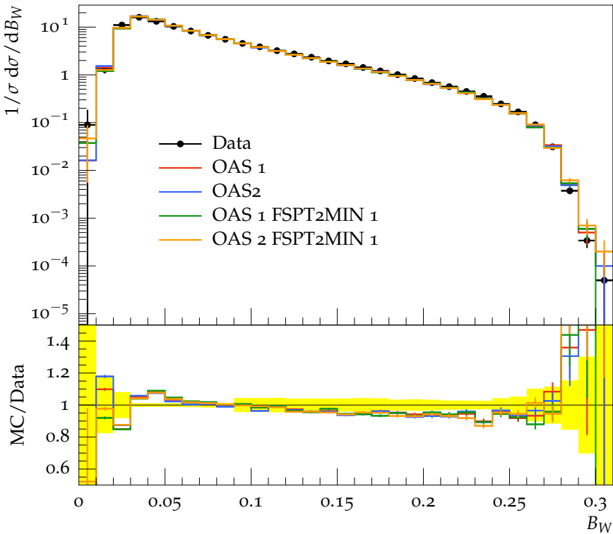
Wide jet broadening ( E_{\text{CMS}} = 91.2 \text{ GeV} )
