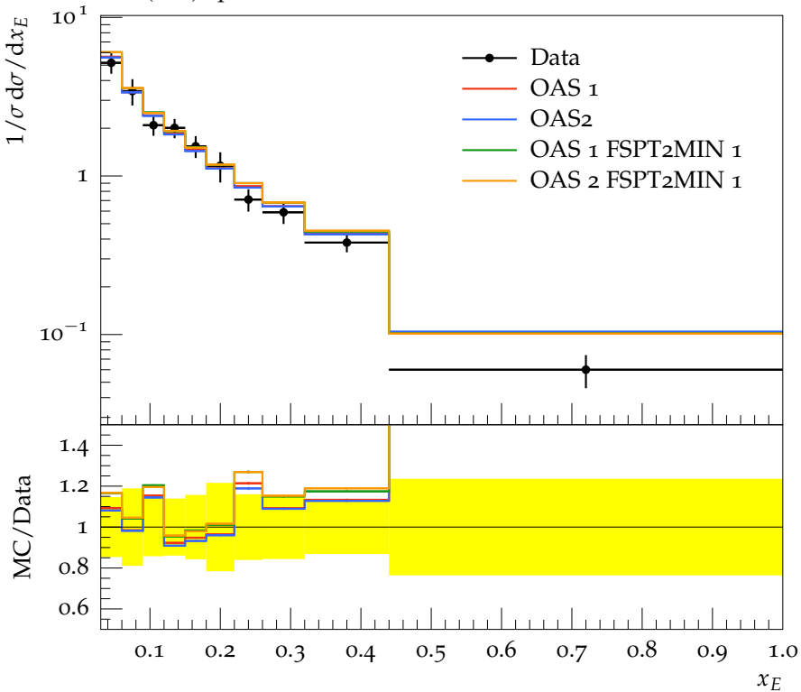
K^{*\pm}(892) spectrum
