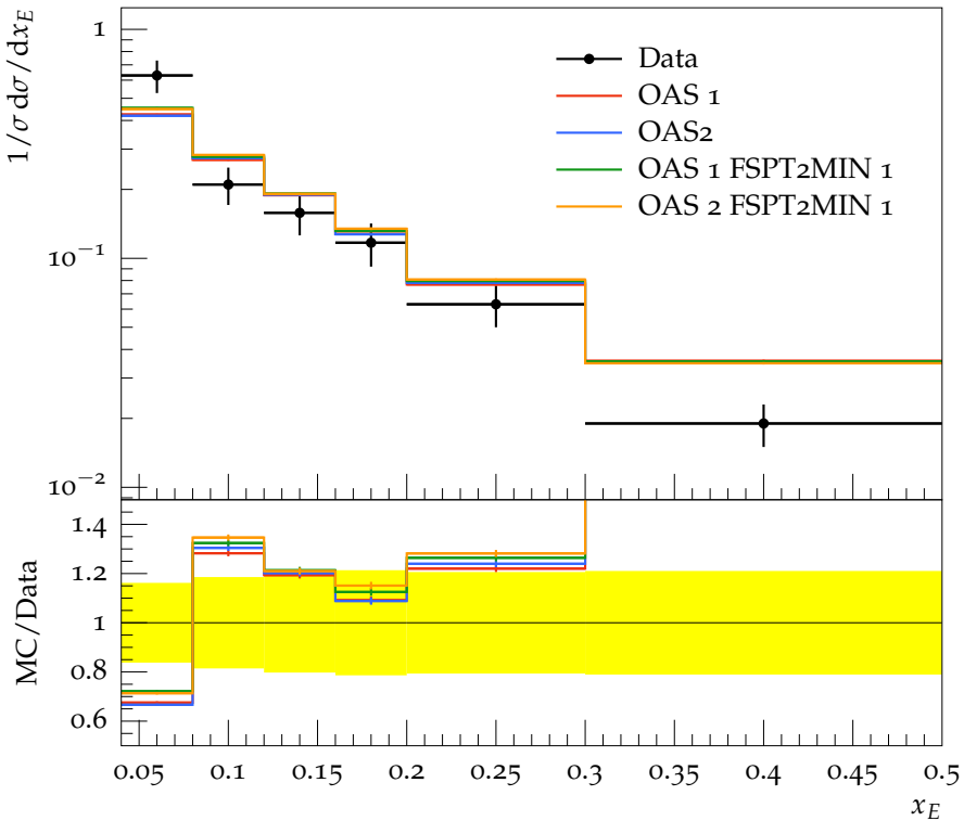
\Sigma^\pm(1385) spectrum
