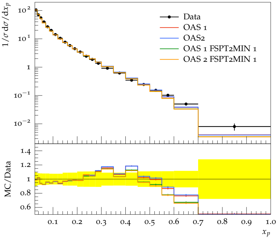
\pi^0 spectrum
