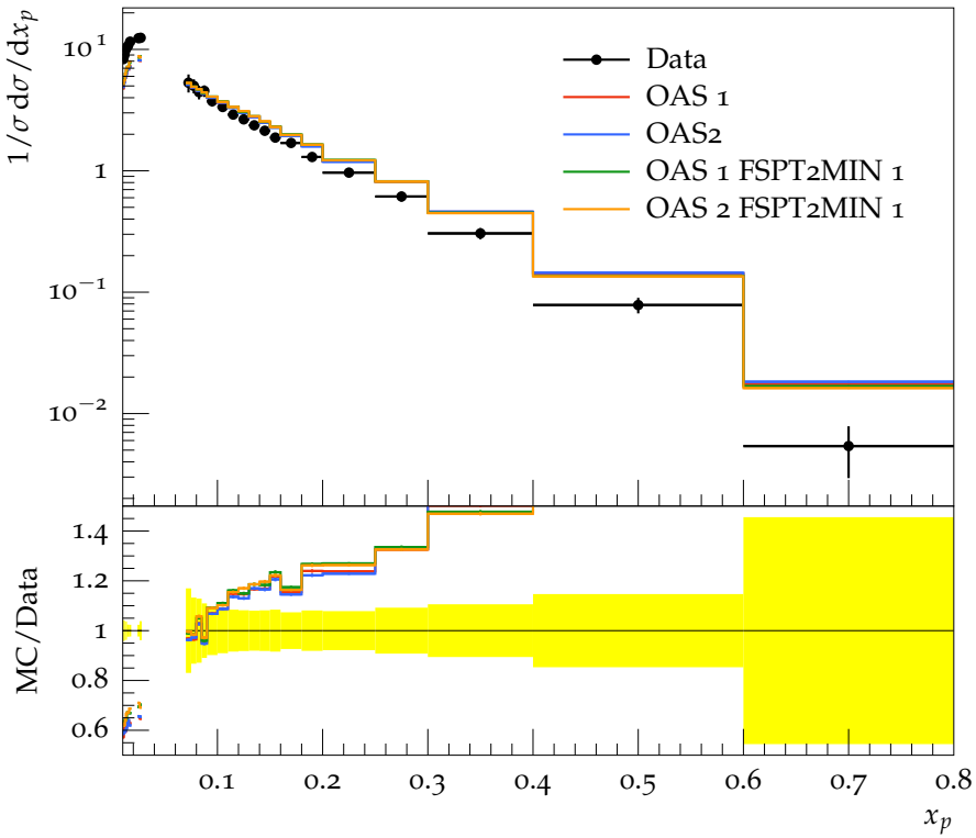
p spectrum
