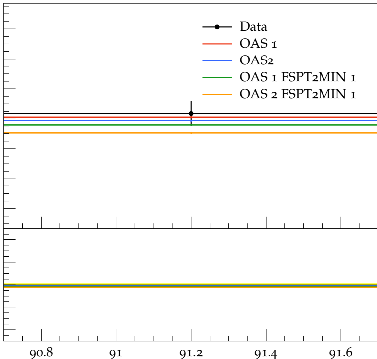
Mean charged multiplicity for rapidity |Y| < 1.0
