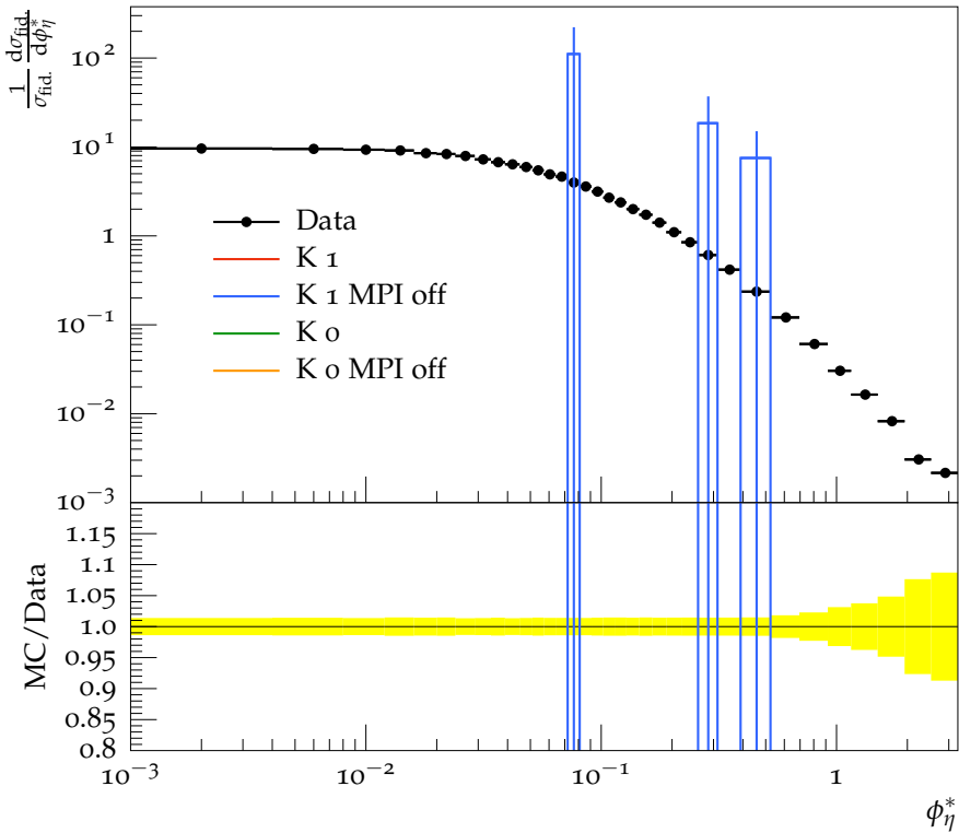
\phi_\eta^* spectrum, Z \rightarrow ee (dressed), |y_Z| \geq 1.6
