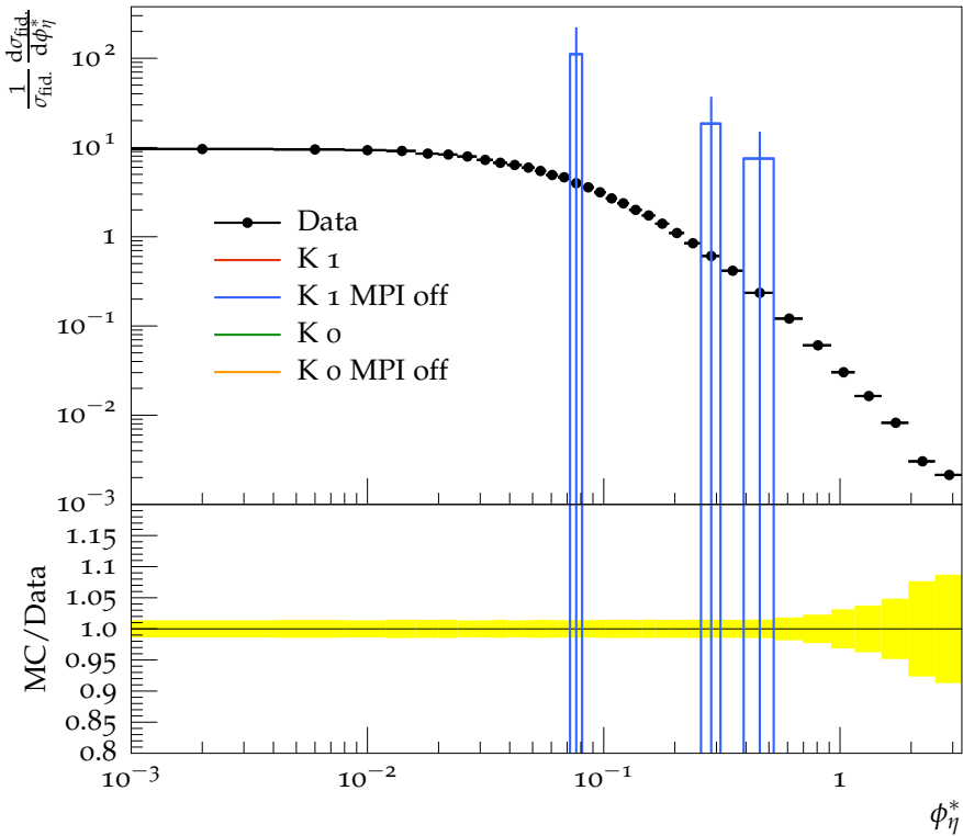
\phi_\eta^* spectrum, Z \rightarrow ee (bare), |y_Z| \geq 1.6
