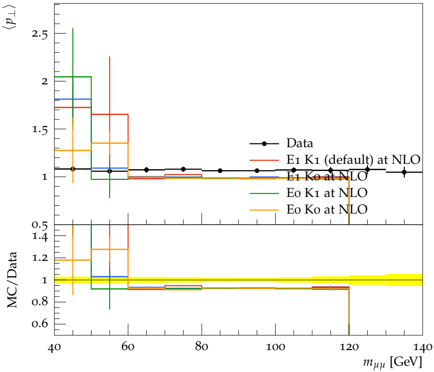
Towards + transverse \langle p_{\perp} \rangle vs m_{\mu\mu} , p_{\perp}^{\mu\mu} < 5 GeV
